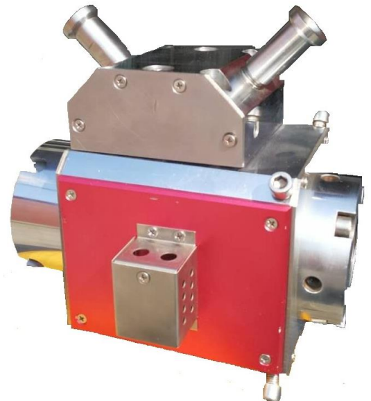
SKIN/FOAM/SKIN CROSSHEAD 0.4 – 5.0 MM PRODUCT OD
